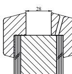
Glaslatten Fire Proof 30
