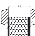
Glaslatten Fire Proof 60
