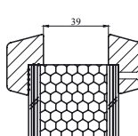
Glaslatten Fire Proof 60
